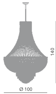
Washington sospensione Ø 100 cm Ø 100 cm - H 140 cm 18 x E14 40W
