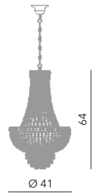
Washington sospensione Ø 40 cm Ø 41 cm - H 64 cm 6 x E14 40W
