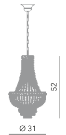
Washington sospensione Ø 30 cm Ø 31 cm - H 52 cm 5 x E14 40W
