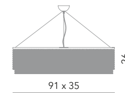
lampadario ovale 6L L 91 x 35 cm - H 26 cm 6 x G9 60W
