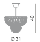
Washington sospensione Ø 30 cm Ø 31 cm - H 40 cm 3 x E14 40W
