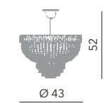
Borbone sospensione Ø 40 cm Ø 43 cm - H 52 cm 4 x E14 40W
